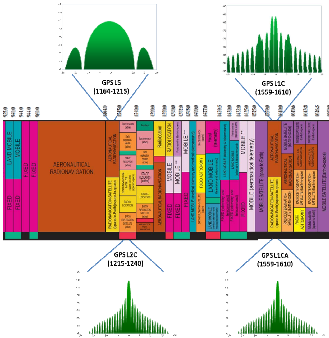
Figure 1-1 Civil GPS Signals and the Spectrum Environment
