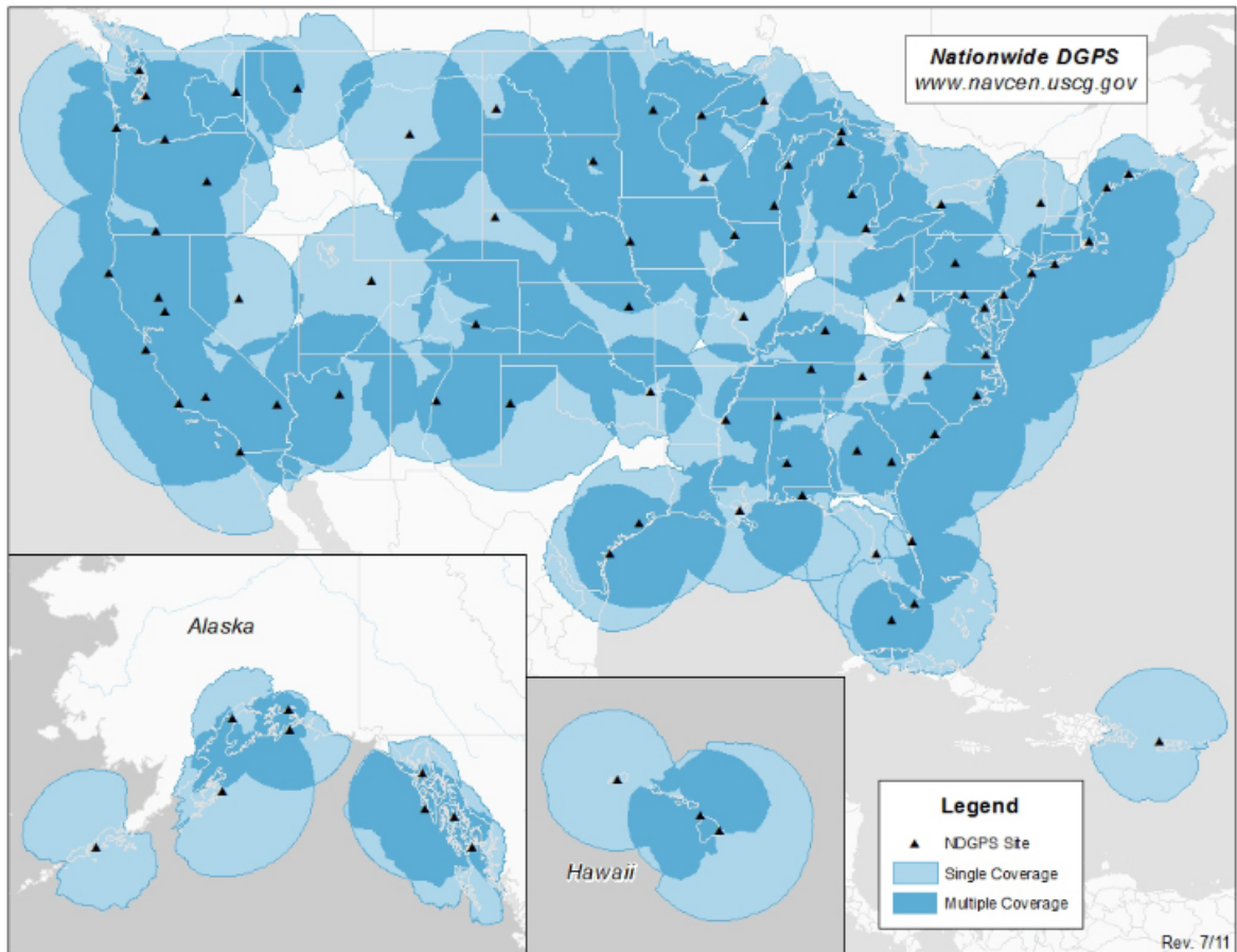
Figure A-6 NDGPS Signal Coverage
