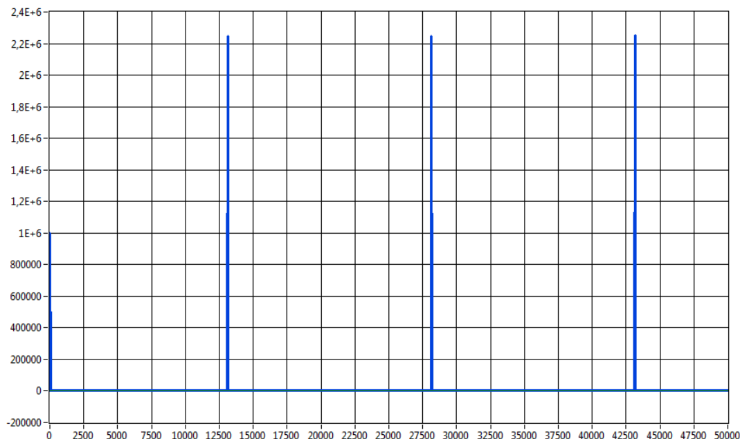
Figure 10 Consumption [µA] vs. Samples, samples taken every 12 ms.
