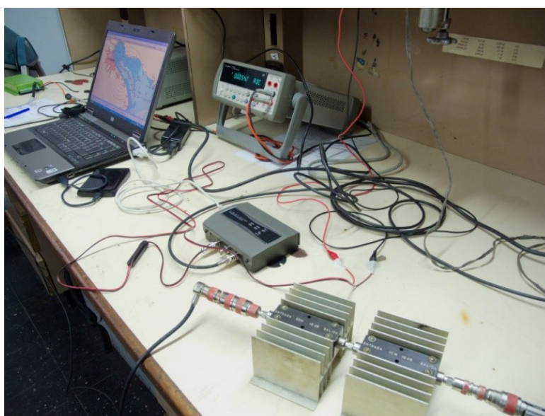
Figure 12 Bench test
