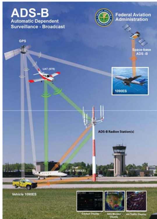
Figure A-7 ADS-B Architecture
