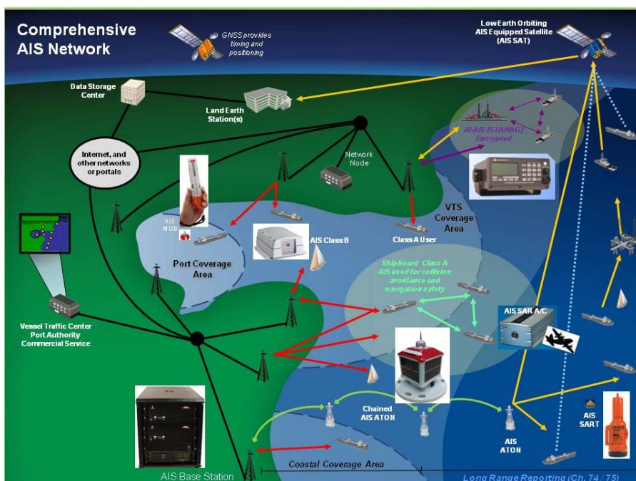
Figure 3 Representation of some types of AIS Stations
