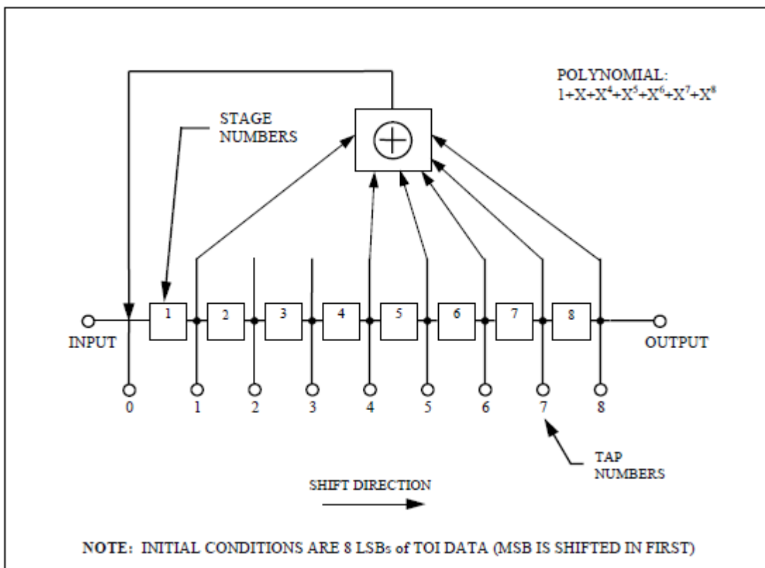
Figure 3.2-4. BCH (51, 8) Code Generator
