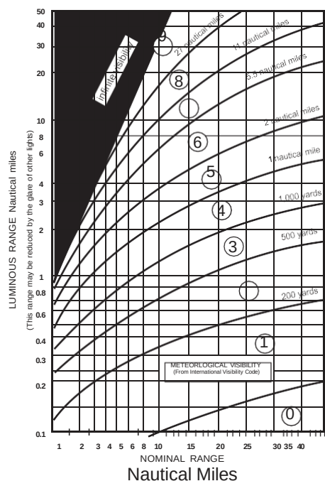
METEOROLOGICAL VISIBILITY (From International Visibility Code)
