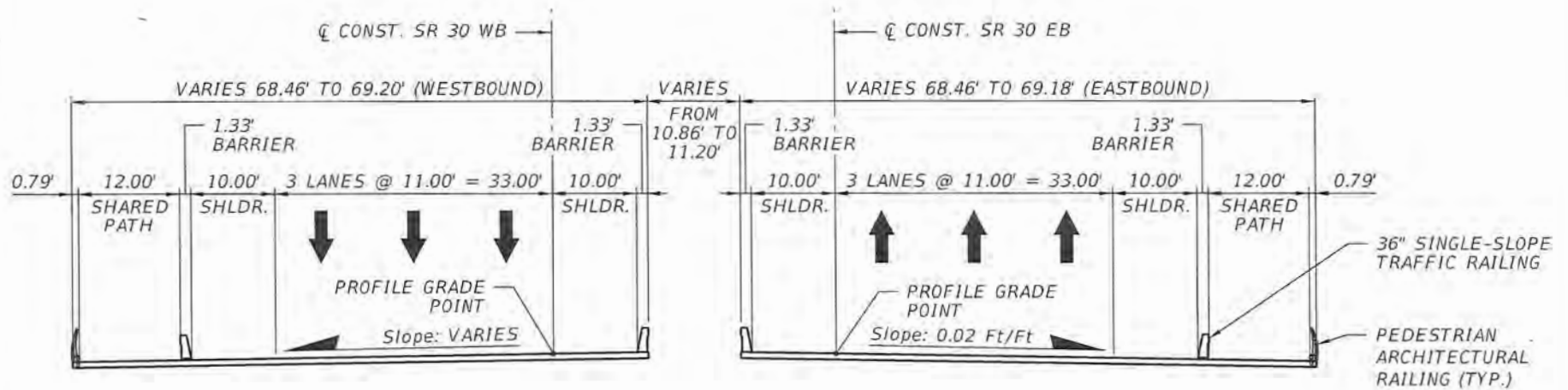
TYPICAL SECTION - PROPOSED BRIDGES (LOOKING AHEAD STATION)
